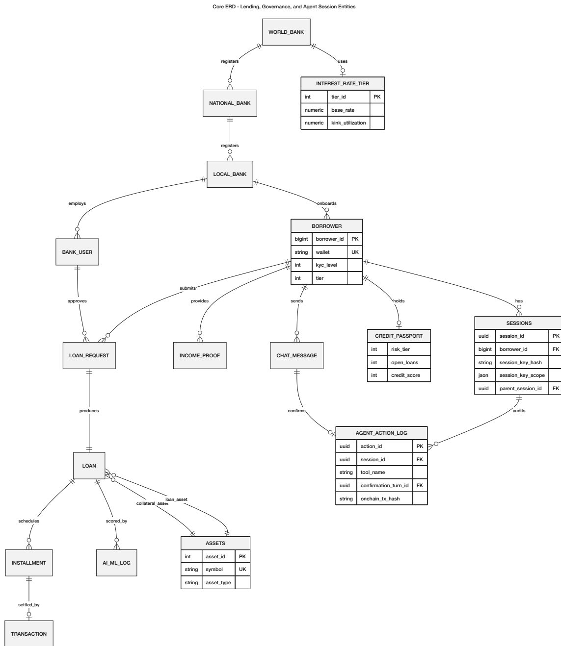
Figure 3.5: Core system graph showing entity relationships across the four-tier banking hierarchy ( \text{WORLD\_BANK} \rightarrow \text{NATIONAL\_BANK} \rightarrow \text{LOCAL\_BANK} \rightarrow \text{BANK\_USER} ), the central BORROWER entity, and the lending-lifecycle sub-graph ( LOAN_REQUEST , LOAN , INSTALLMENT , TRANSACTION , INCOME_PROOF , CHAT_MESSAGE , AI_ML_LOG , CREDIT_PASSPORT ).
