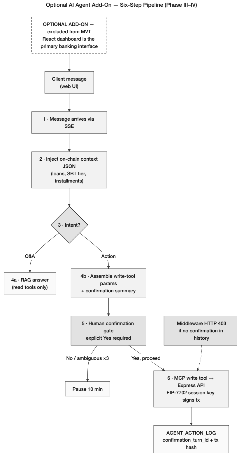
Figure 3.13: Optional AI agent add-on (Phase III–IV, excluded from MVT): six-step pipeline with on-chain context injection, read/write routing, mandatory human confirmation gate, MCP write-tool execution, and AGENT_ACTION_LOG audit trail. React dashboard remains the primary interface.
