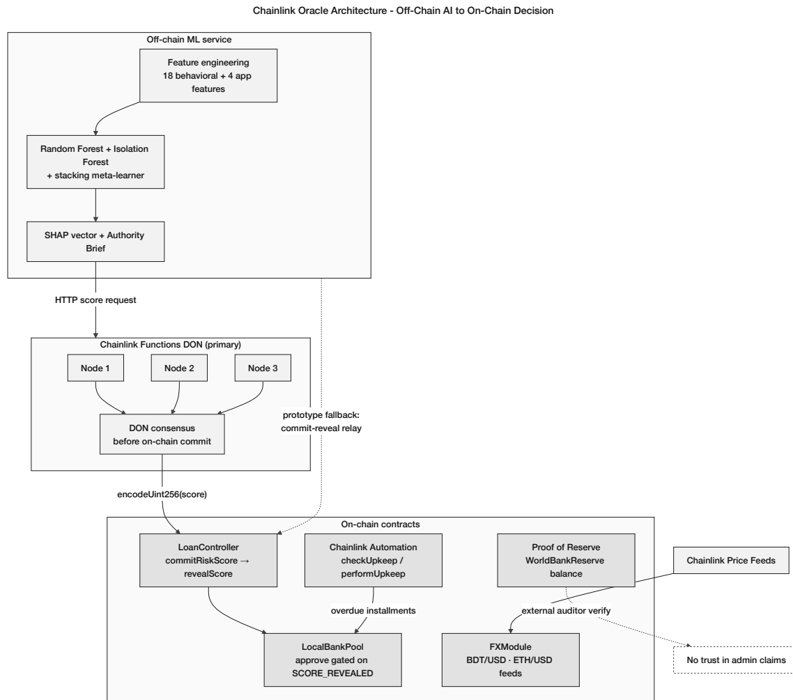
Figure 3.4: Chainlink oracle architecture: (a) off-chain ML feature engineering and SHAP explainability, (b) Chainlink Functions DON consensus for risk-score commitment, (c) on-chain LoanController state machine gating approval on SCORE_REVEALED, with Chainlink Automation, Price Feeds, and Proof of Reserve. The commit-reveal relay remains the prototype-phase fallback until Phase III wiring is complete.
