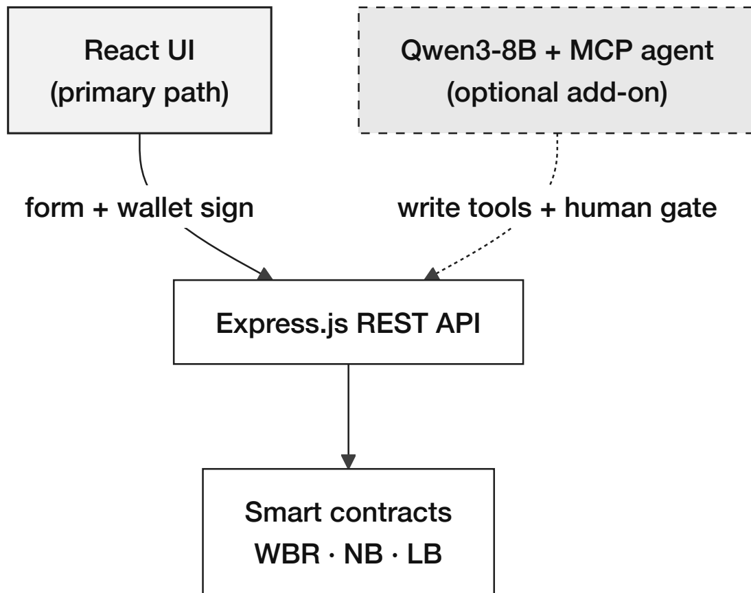
Figure 4.8: Optional conversational agent add-on: React UI (primary path) and MCP agent (alternate path) both call the same Express.js API and smart contracts; the agent does not gate core banking operations.
