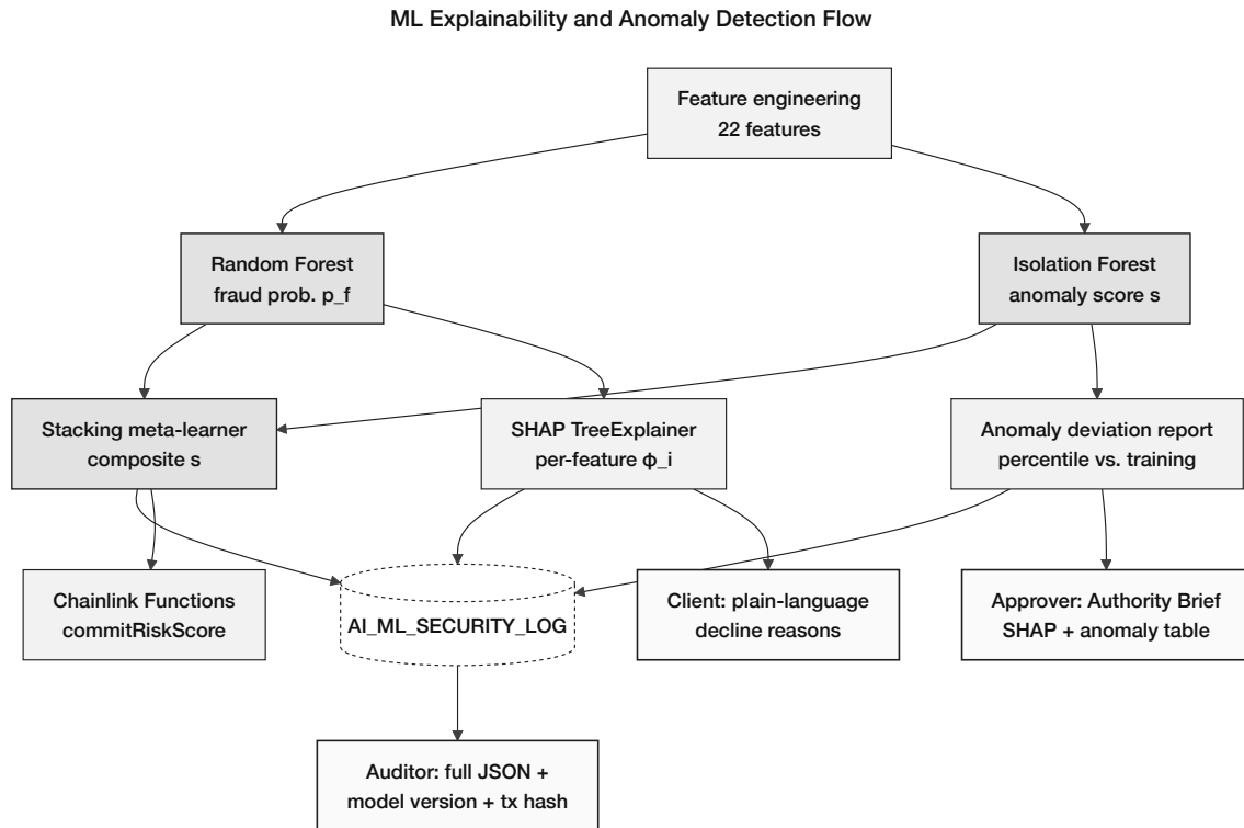
Figure 4.3: Explainability and anomaly-detection flow: feature engineering \rightarrow Random Forest ( p_f ) + Isolation Forest (anomaly s ) \rightarrow stacking meta-learner \rightarrow SHAP + deviation report \rightarrow three audiences (client, approver, auditor) \rightarrow oracle commit; human approver retains final disbursement authority.
