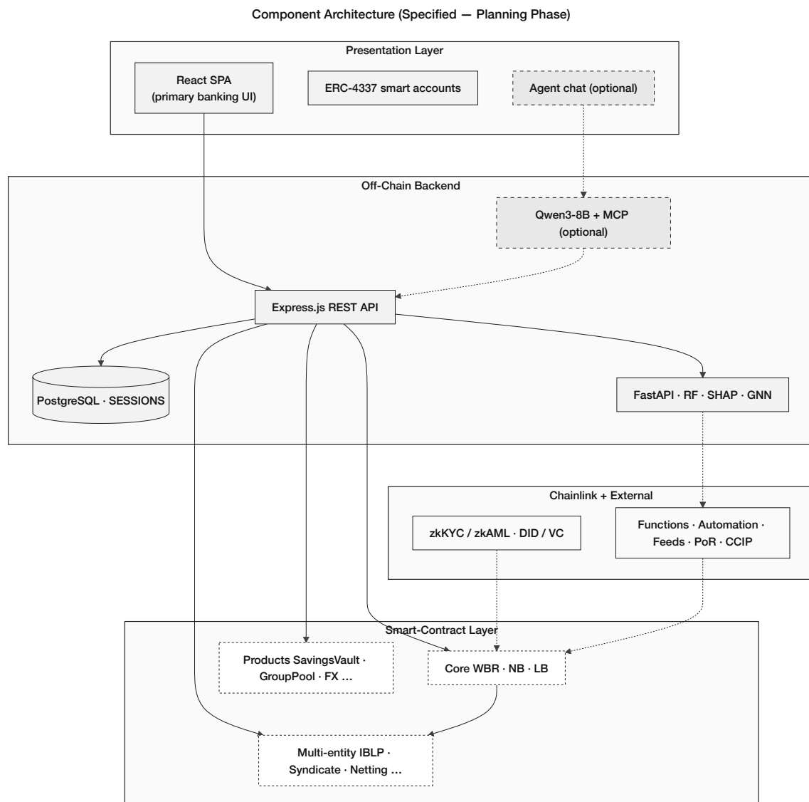
Figure 3.2: Component diagram (planning phase): React UI is the primary path; optional MCP agent (dashed) shares the Express.js API; smart contracts and Chainlink integrations are specified for Phase I–IV deployment.
