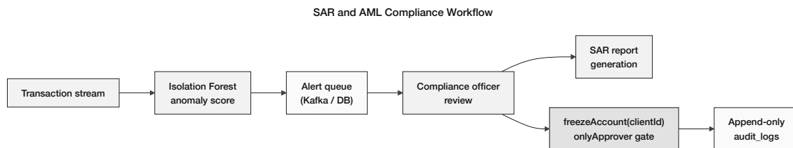
Figure 3.29: SAR and AML compliance workflow: Isolation Forest anomaly detection, compliance officer review queue, optional SAR report generation, on-chain freezeAccount via onlyApprover, and append-only audit_logs record.
