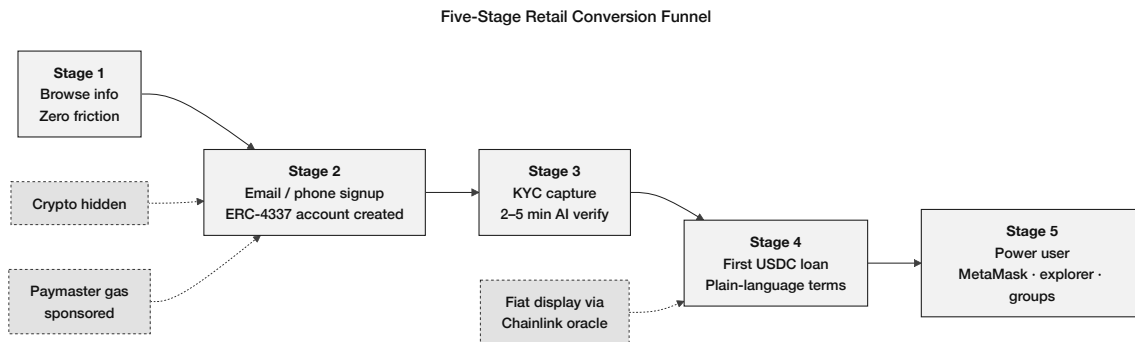
Figure 3.12: Five-stage retail onboarding funnel: progressive disclosure from zero-friction browsing through wallet or optional ERC-4337 account creation, KYC, first USDC loan with optional fiat-equivalent display, to power-user and group-lending modes.
