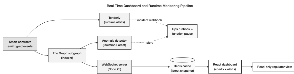
Figure 4.4: Real-time dashboard and runtime monitoring pipeline: smart contracts emit typed events; The Graph indexes them and pushes to a Node WebSocket server which renders the React dashboard via a Redis snapshot. Tenderly runtime alerts and an Isolation-Forest anomaly detector feed the operations runbook with the granular-pause control surface of Section 3.19.
