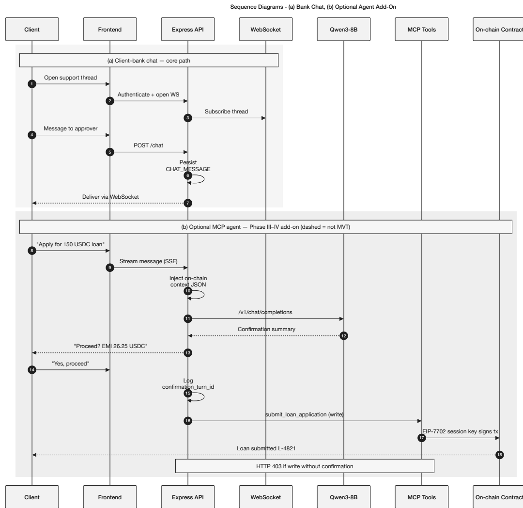
Figure 3.24: Sequence diagrams: (a) client–bank chat over an authenticated WebSocket, and (b) optional MCP agent pipeline (on-chain context injection, read/write routing, human confirmation gate, EIP-7702 session-key signing; Phase III–IV add-on).
