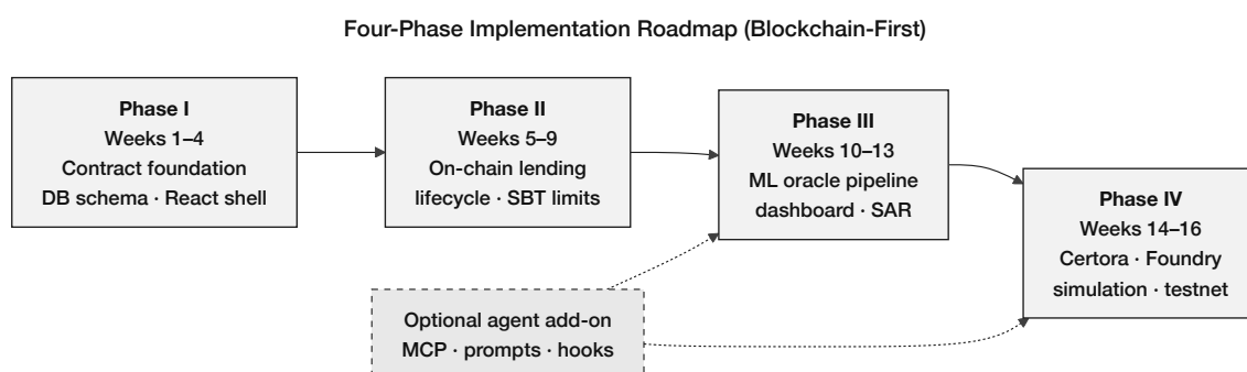
Figure 4.7: Four-phase implementation roadmap (blockchain-first): Phase I contract foundation, Phase II on-chain lending lifecycle, Phase III ML oracle pipeline, Phase IV verification and testnet deployment; optional agent add-on spans Phases III–IV (dashed).
