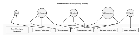
Figure 3.10: Actor permission matrix (primary actions): clients submit loans and pay installments via the React UI (or optionally via the MCP agent); Local Bank approvers approve and freeze accounts; National and World Bank admins set rates and reserve parameters; the optional AI Agent may call read tools freely and write tools only after human confirmation (†).
