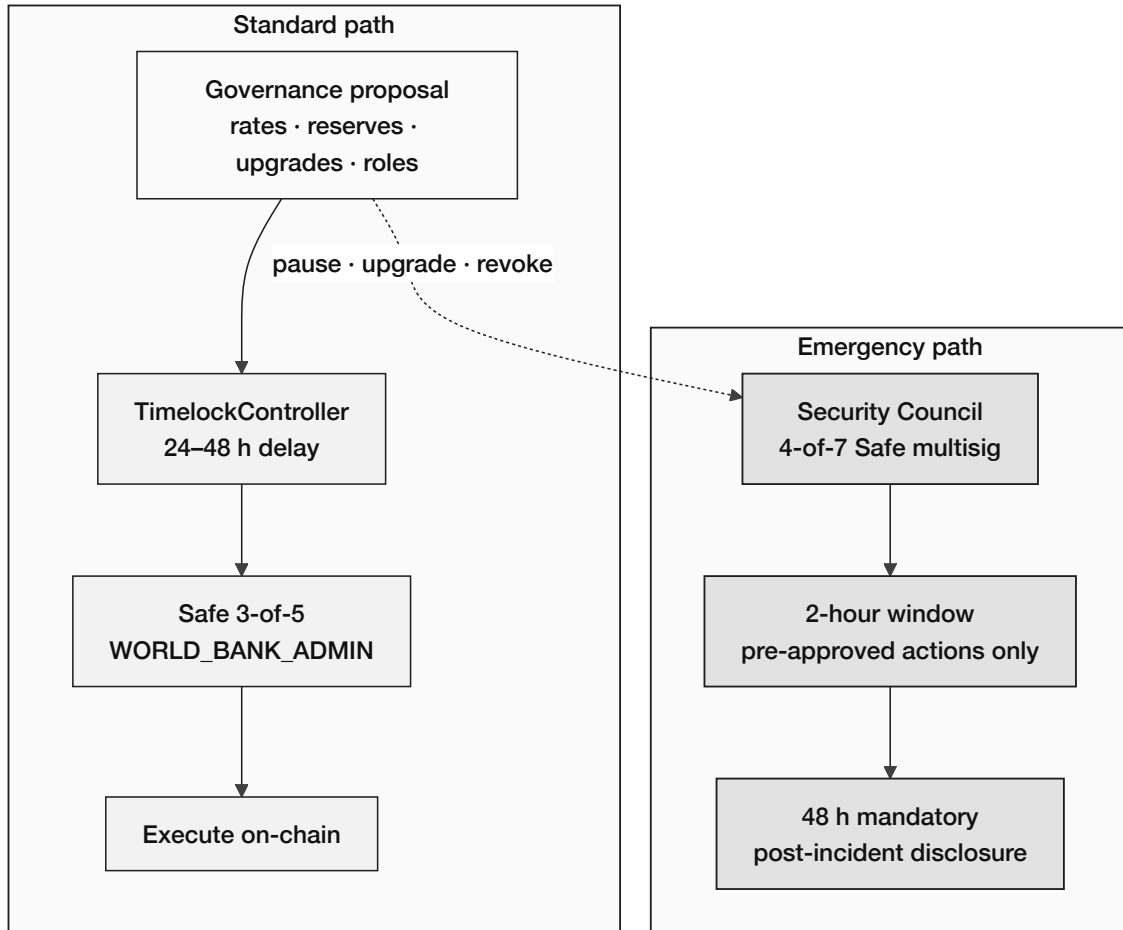
Figure 3.28: Governance dual-path: (a) standard TimeLock-gated parameter changes and upgrades via Safe 3-of-5, and (b) Security Council emergency path (4-of-7) for pre-approved pause, upgrade, and role-revocation actions within a 2-hour window with mandatory 48-hour disclosure.
