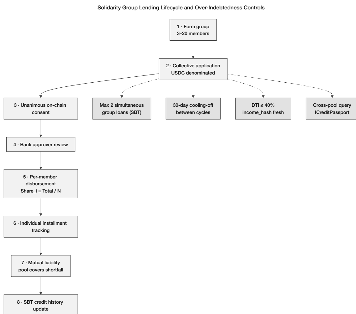
Figure 3.27: Solidarity group lending lifecycle: eight on-chain stages from group formation through mutual-liability enforcement and SBT credit-history update, with over-indebtedness controls (simultaneous-loan cap, cooling-off period, DTI ceiling, and cross-pool ICreditPassport query).
