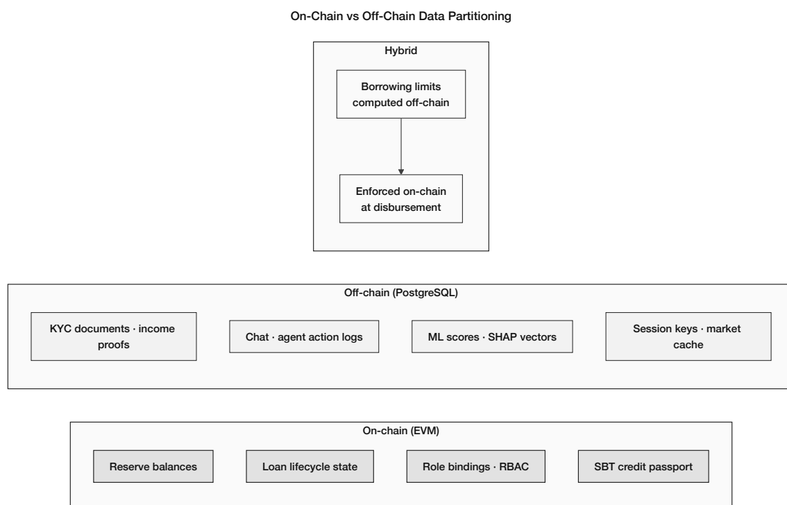
Figure 3.8: On-chain versus off-chain data partitioning: reserve balances, loan state, and role bindings on the EVM; KYC documents, agent logs, and ML scores in PostgreSQL; borrowing limits computed off-chain and enforced on-chain at disbursement.
