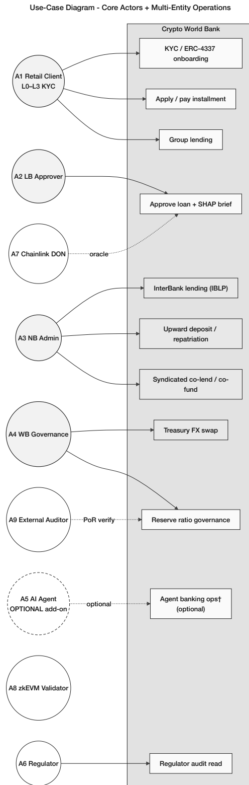
Figure 3.16: Use-case diagram reflecting the nine-actor taxonomy of Table 3.17: four core primary actors (A1–A4), optional add-on AI Agent (A5, dashed), and four secondary actors (A6–A9). Highlighted use cases cover multi-entity operations (IBLP, upward deposit, syndicated co-lend, treasury FX); optional agent banking ops (UC10) are excluded from MVT.
