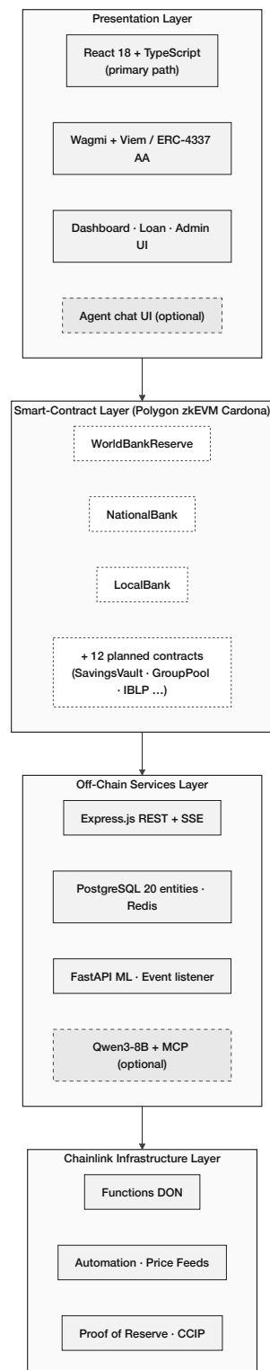
Figure 3.1: Four-layer decentralised application architecture (blockchain-first): presentation (React 18, TypeScript, Wagmi/Viem); smart-contract layer on the EVM (World Bank Reserve, National Bank, Local Bank + twelve planned modules); off-chain services (Express REST API, PostgreSQL, FastAPI ML, Chainlink integration, Redis); Chainlink infrastructure (Functions, Automation, Price Feeds, Proof of Reserve). Optional add-on: MCP agent UI (dashed).
