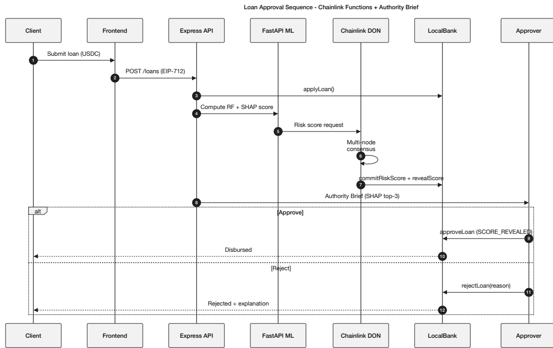
Figure 3.21: Sequence diagram for the loan-approval flow with reject alternative: the client submits an EIP-712 signed request, the ML oracle returns a SHAP-explained score via commit-reveal, and the approver either approves (revealing the commit) or rejects (with reason logged on-chain).
