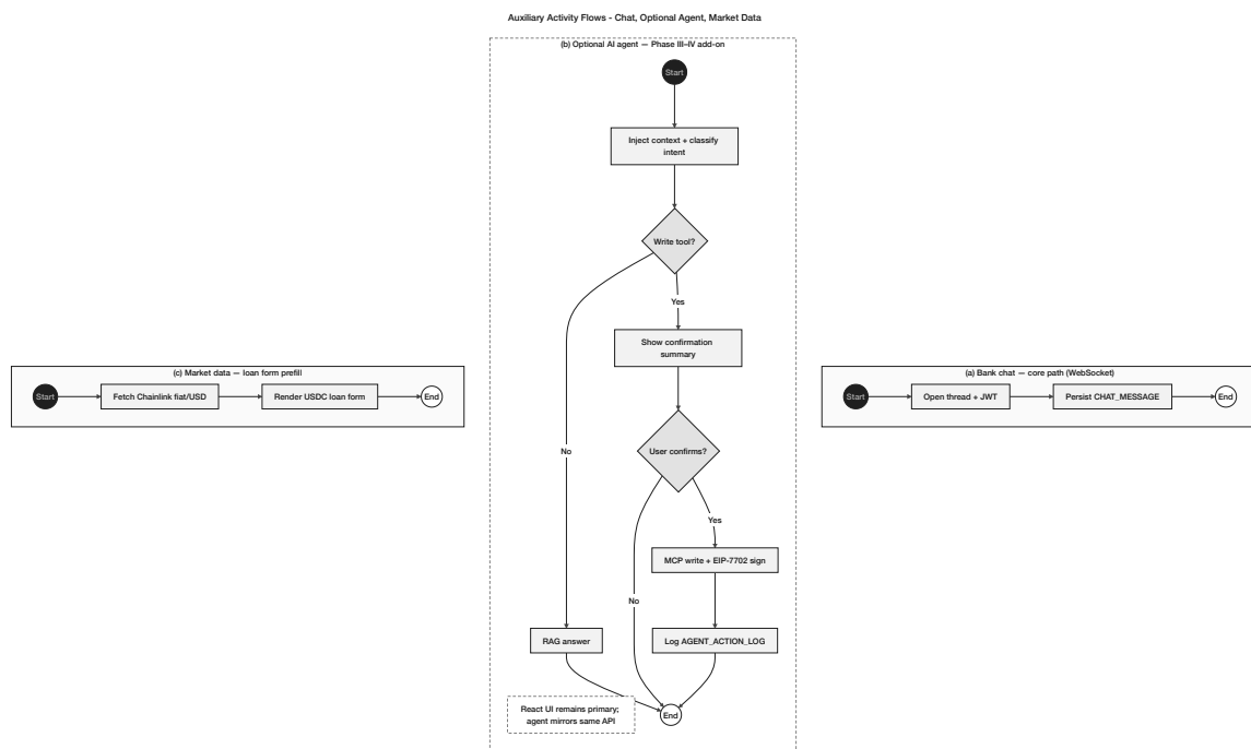
Figure 3.19: Auxiliary activity flows: (a) client–bank chat over authenticated WebSocket, (b) optional MCP agent Q&A with on-chain context injection and confirmation gate (Phase III–IV), (c) live market-data retrieval and pre-filled loan sizing.
