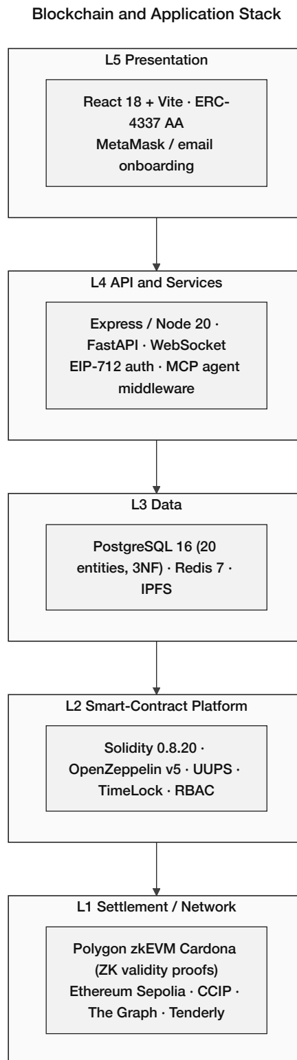
Figure 3.3: Layered blockchain and application stack: L1 settlement (Polygon zkEVM Cardona for retail, Ethereum Sepolia for institutional, plus Chainlink CCIP bridge, The Graph indexer, and Tenderly monitor); L2 smart-contract platform (Solidity 0.8.20, OpenZeppelin v5, UUPS, TimeLock, RBAC); L3 data (PostgreSQL 16 in 3NF, Redis, IPFS); L4 API and services (Express, FastAPI, WebSocket, EIP-712); L5 presentation (React + ERC-4337 account abstraction).
